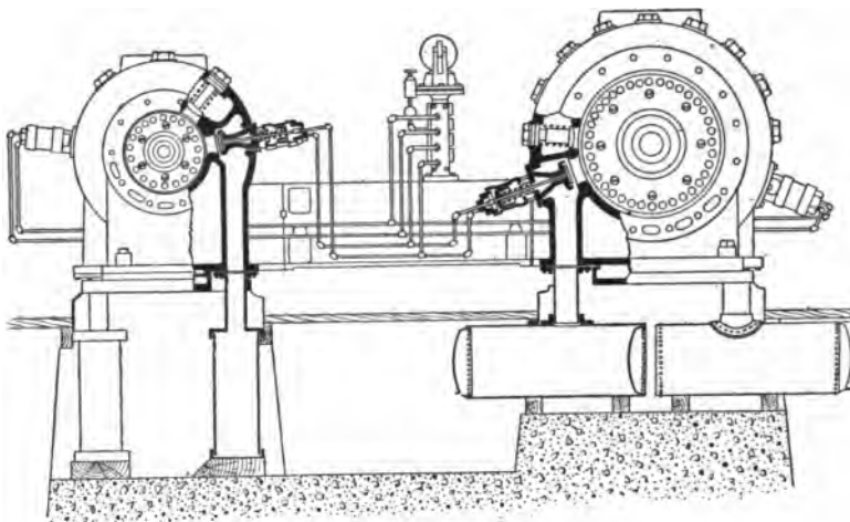
FIG. 84.—Clearance unloader.
